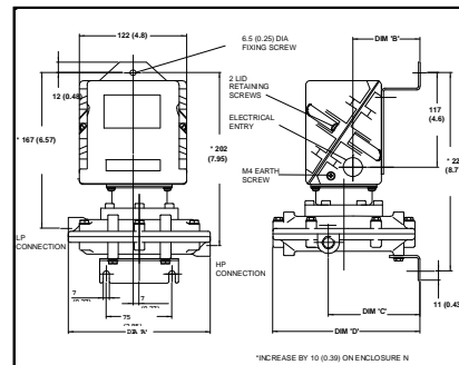
FIG 6 MODELS W, N 306, 386 RANGES B2 TO C6
