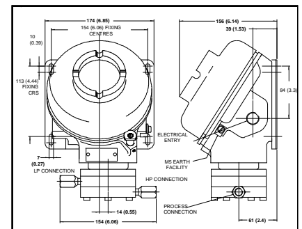
FIG 9 MODELS H, K 306, 386 RANGES E1 TO J0
