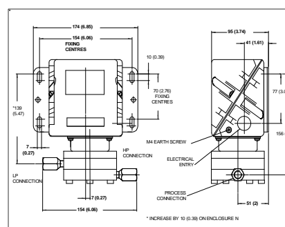
FIG 8 MODELS W, N 306, 386 RANGES E1 TO J0
