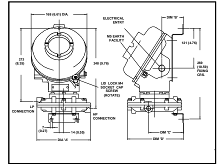
FIG 7 MODELS H, K 306, 386 RANGES B2 TO C6
