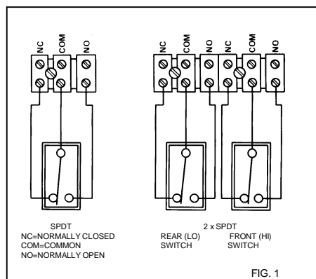
FIG.1 shows the state of electrical contacts at atmospheric pressure.
